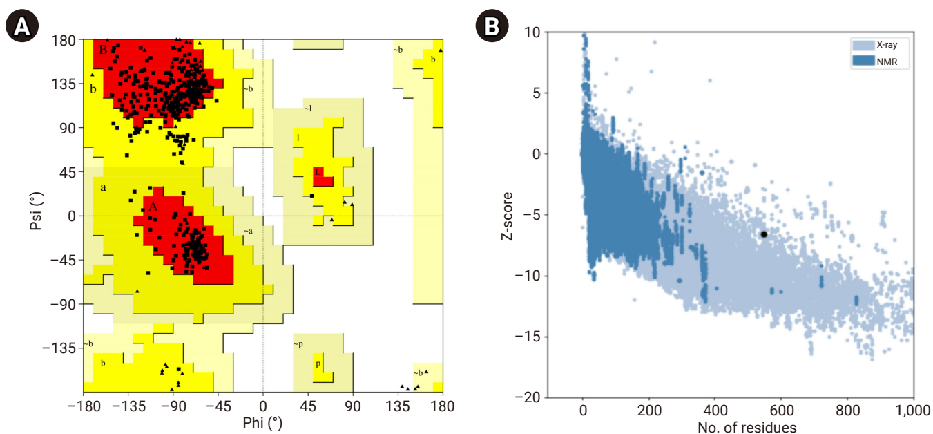
Figure S1. Tertiary structure quality assessment graphs of the 50S ribosomal protein L7/L12-adjuvanted vaccine construct structures in Procheck (A) and ProSA-web (B). NMR, nuclear magnetic resonance.
