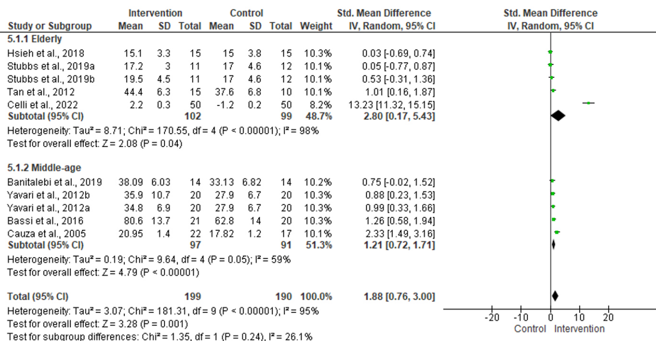
Figure S7. Effect of resistance training on VO_2 peak.
