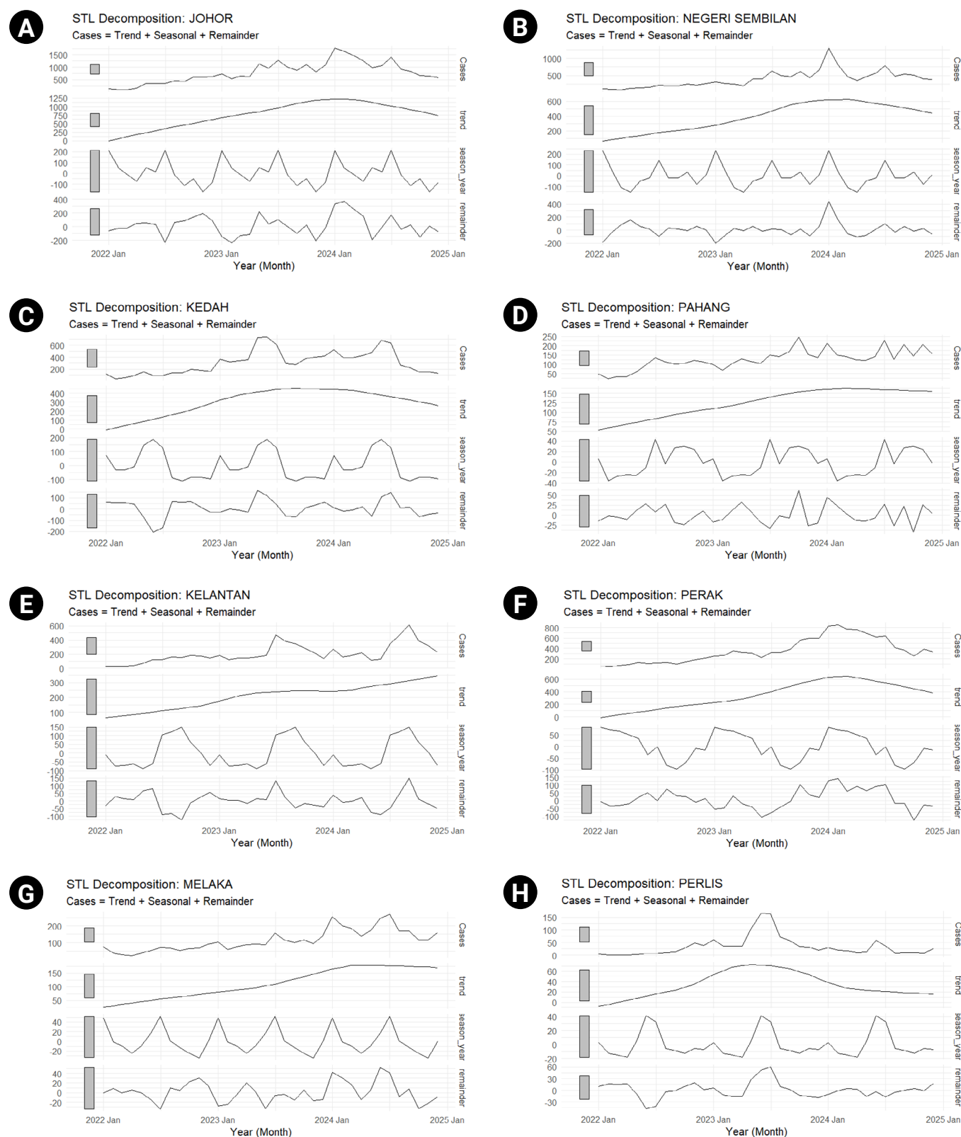
Figure S1. Seasonal-trend decomposition using LOESS (STL) decomposition plot for every state. Panels show observed cases (top), long-term trend, seasonal component, and remainder. (A) Johor, (B) Negeri Sembilan, (C) Kedah, (D) Pahang, (E) Kelantan, (F) Perak, (G) Melaka, (H) Perlis, (I) Pulau Pinang, (J) Terengganu, (K) Selangor, (L) Sarawak, (M) Sabah, (N) Wilayah Persekutuan. (Continued on the next page.)
