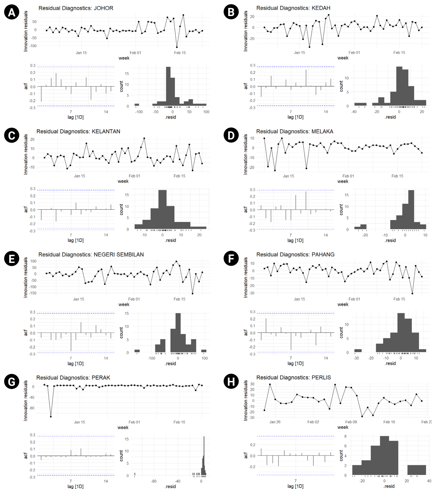
Figure S3. Residual diagnostic for SARIMA/ARIMA models for every state (ACF and histogram). ARIMA, autoregressive integrated moving average; SARIMA, seasonal ARIMA; ACF, autocorrelation function. (A) Johor, (B) Kedah, (C) Kelantan, (D) Melaka, (E) Negeri Sembilan, (F) Pahang, (G) Perak, (H) Perlis, (I) Pulau Pinang, (J) Sabah, (K) Sarawak, (L) Selangor, (M) Terengganu, (N) Wilayah Persekutuan. (Continued on the next page.)
